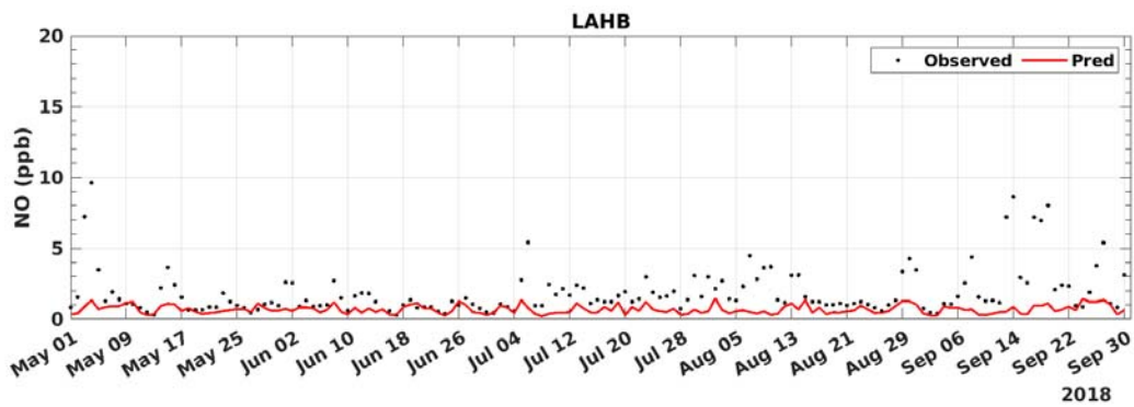
FIGURE B-12: 2018 DAILY AVERAGED NO MODEL PREDICTION AND MEASUREMENT COMPARISON AT LA HABRA
