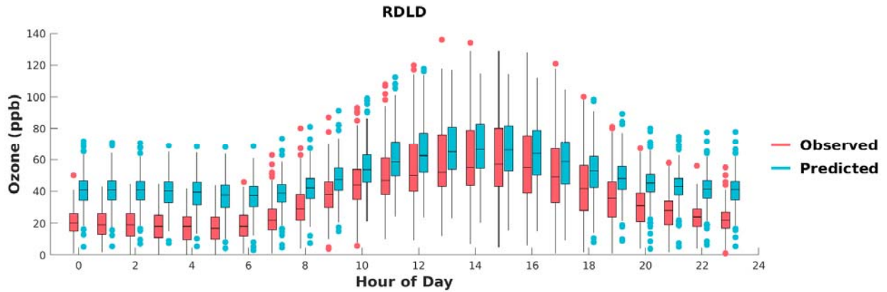
FIGURE F-23: BOX PLOTS OF OBSERVED VS. PREDICTED HOURLY OZONE DURING MAY 1 ST TO SEPTEMBER 30 TH , 2018, AT REDLANDS. HORIZONTAL LINES INDICATE 25 TH , 50 TH (MEDIAN), AND 75 TH PERCENTILES.
