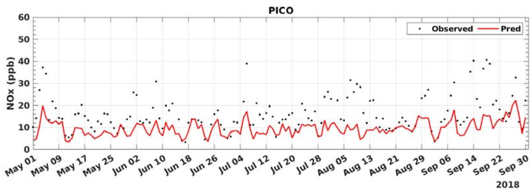
FIGURE D-14: 2018 DAILY AVERAGED NOX MODEL PREDICTION AND MEASUREMENT COMPARISON AT PICO RIVERA
