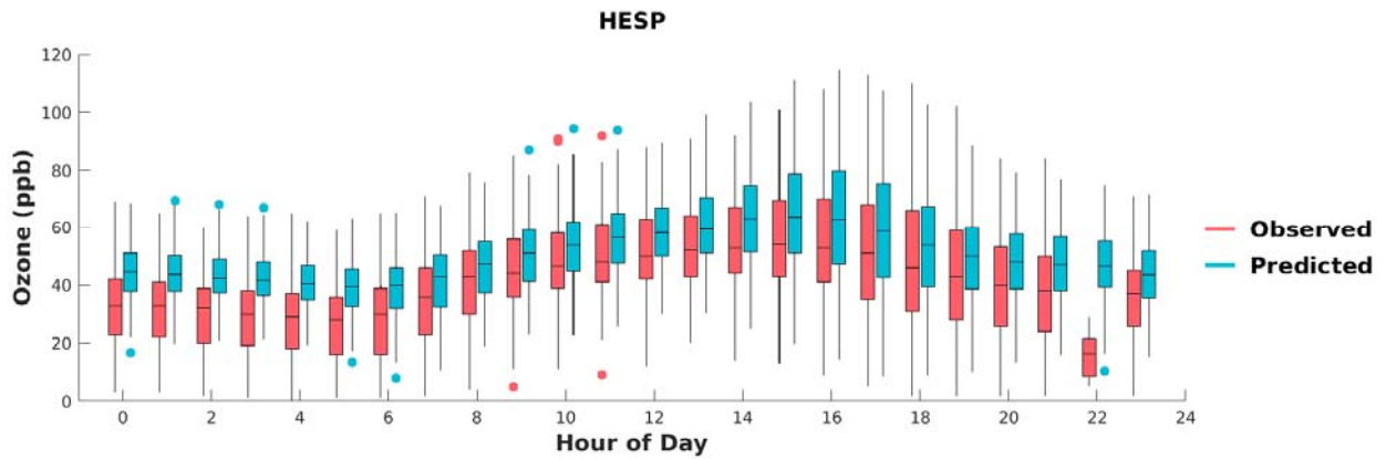
FIGURE F-11: BOX PLOTS OF OBSERVED VS. PREDICTED HOURLY OZONE DURING MAY 1 ST TO SEPTEMBER 30 TH , 2018, AT HESPERIA. HORIZONTAL LINES INDICATE 25 TH , 50 TH (MEDIAN), AND 75 TH PERCENTILES.
