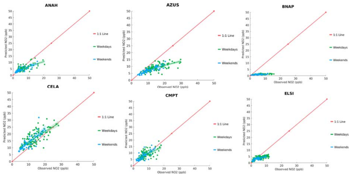
FIGURE M-1: SCATTER PLOT OF OBSERVED VS. PREDICTED DAILY AVERAGE NO2 DURING MAY 1 ST TO SEPTEMBER 30 TH , 2018, AT ANAHEIM (ANAH), AZUSA(AZUS), BANNING (BNAP), CENTRAL LOS ANGES (CELA), COMPTON (CMPT), AND LAKE ELSIONOR (ELSI). GREEN AND BLUE LINES INDICATE GENERAL LINEAR MODEL FIT WITH 95% CONFIDENCE INTERVAL (SHADED AREA). THE RED LINE INDICATES 1:1 LINE.
