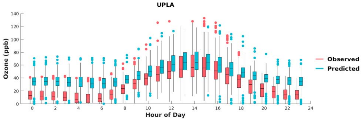
FIGURE F-29: BOX PLOTS OF OBSERVED VS. PREDICTED HOURLY OZONE DURING MAY 1 ST TO SEPTEMBER 30 TH , 2018, AT UPLAND. HORIZONTAL LINES INDICATE 25 TH , 50 TH (MEDIAN), AND 75 TH PERCENTILES.
