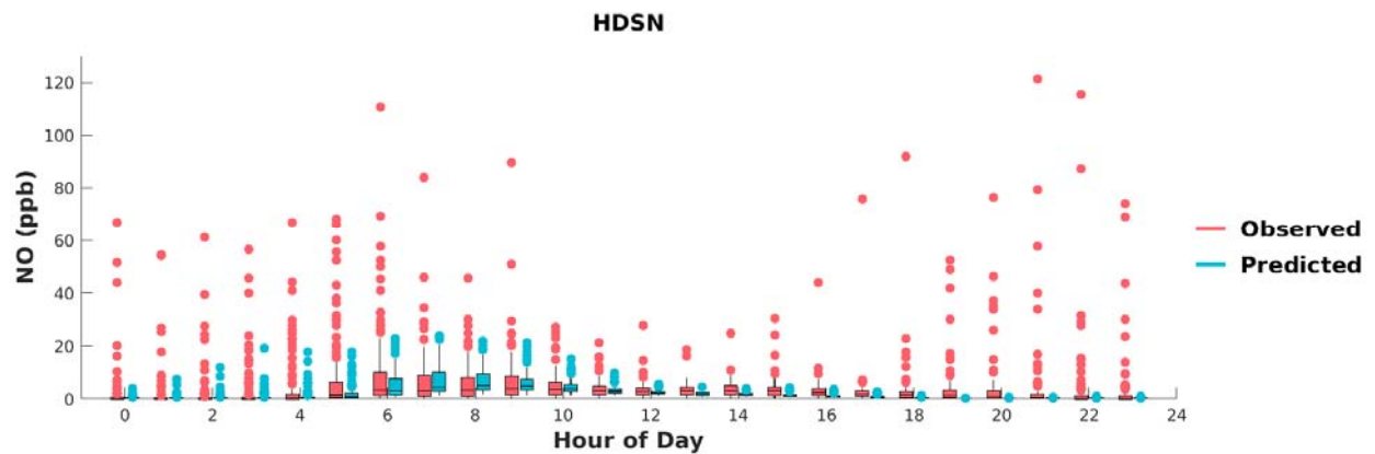
FIGURE G-9: BOX PLOTS OF OBSERVED VS. PREDICTED HOURLY NO DURING MAY 1 ST TO SEPTEMBER 30 TH , 2018, AT HUDSON. HORIZONTAL LINES INDICATE 25 TH , 50 TH (MEDIAN), AND 75 TH PERCENTILES.
