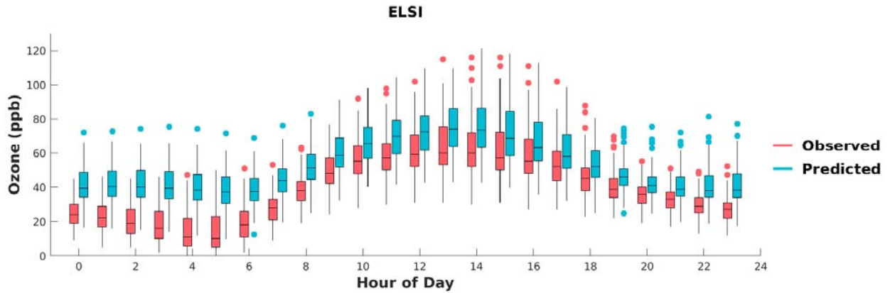
FIGURE F-7: BOX PLOTS OF OBSERVED VS. PREDICTED HOURLY OZONE DURING MAY 1 ST TO SEPTEMBER 30 TH , 2018, AT LAKE ELSINORE. HORIZONTAL LINES INDICATE 25 TH , 50 TH (MEDIAN), AND 75 TH PERCENTILES.
