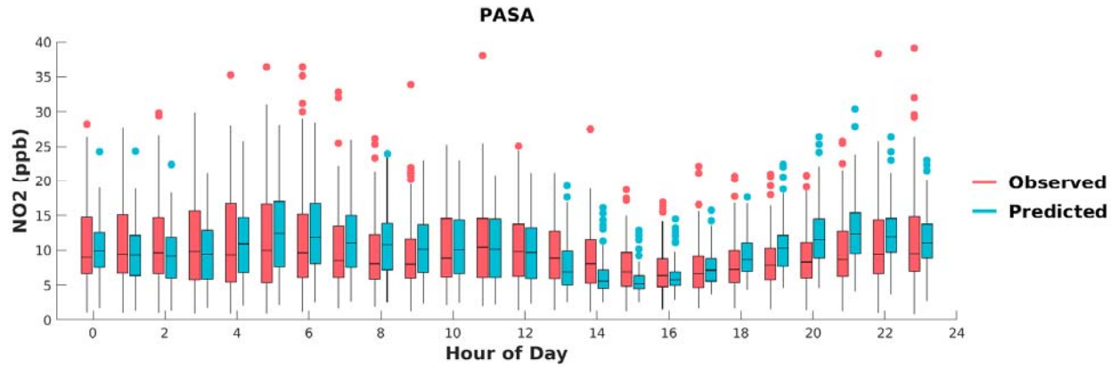
FIGURE H-13: BOX PLOTS OF OBSERVED VS. PREDICTED HOURLY NO 2 DURING MAY 1 ST TO SEPTEMBER 30 TH , 2018, AT PASADENA. HORIZONTAL LINES INDICATE 25 TH , 50 TH (MEDIAN), AND 75 TH PERCENTILES.
