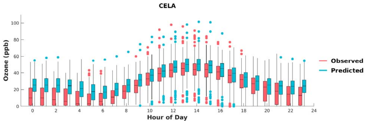
FIGURE F-4: BOX PLOTS OF OBSERVED VS. PREDICTED HOURLY OZONE DURING MAY 1 ST TO SEPTEMBER 30 TH , 2018, AT CENTRAL LOS ANGELES. HORIZONTAL LINES INDICATE 25 TH , 50 TH (MEDIAN), AND 75 TH PERCENTILES.
