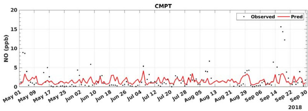
FIGURE B-5: 2018 DAILY AVERAGED NO MODEL PREDICTION AND MEASUREMENT COMPARISON AT COMPTON
