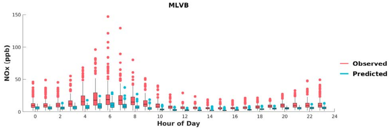
FIGURE I-12: BOX PLOTS OF OBSERVED VS. PREDICTED HOURLY NOX DURING MAY 1 ST TO SEPTEMBER 30 TH , 2018, AT MIRA LOMA VAN BUREN. HORIZONTAL LINES INDICATE 25 TH , 50 TH (MEDIAN), AND 75 TH PERCENTILES.
