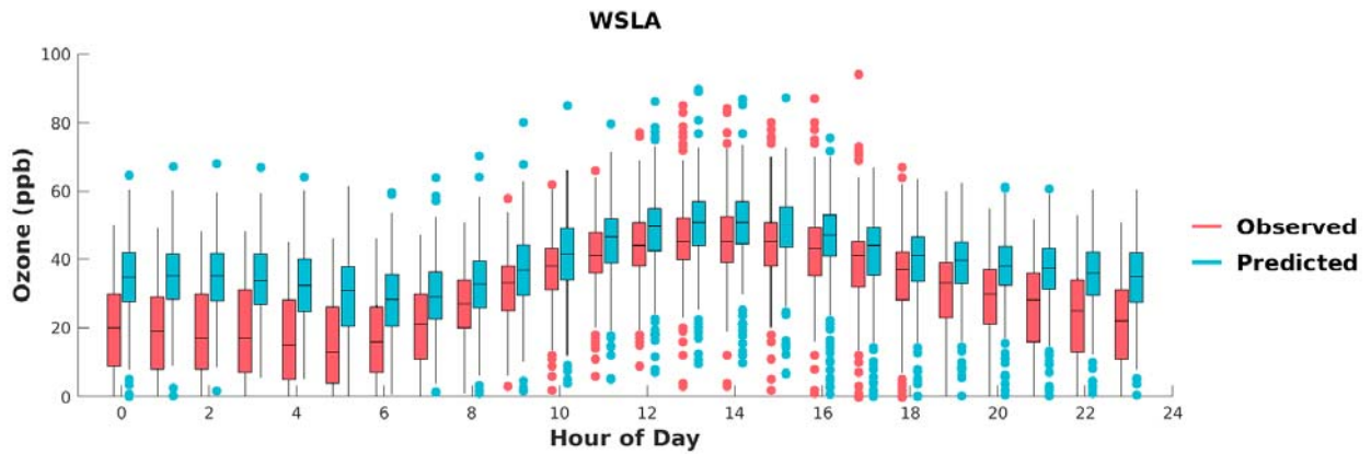
FIGURE F-31: BOX PLOTS OF OBSERVED VS. PREDICTED HOURLY OZONE DURING MAY 1 ST TO SEPTEMBER 30 TH , 2018, AT WEST LOS ANGELES. HORIZONTAL LINES INDICATE 25 TH , 50 TH (MEDIAN), AND 75 TH PERCENTILES.
