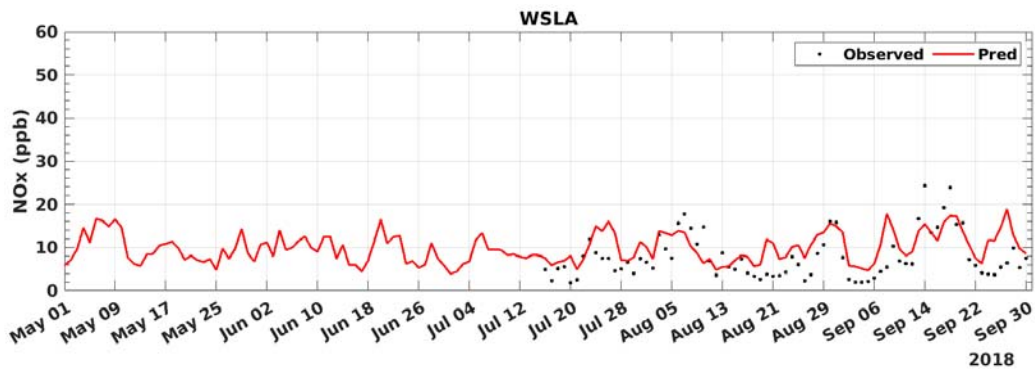
FIGURE D-23: 2018 DAILY AVERAGED NOX MODEL PREDICTION AND MEASUREMENT COMPARISON AT WEST LOS ANGELES
