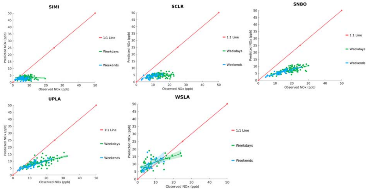
FIGURE N-4: SCATTER PLOT OF OBSERVED VS. PREDICTED DAILY AVERAGE NO x DURING MAY 1 ST TO SEPTEMBER 30 TH , 2018, AT SIMI VALLEY (SIMI), SANTA CLARITA (SCLR), SAN BERNARDION (SNBO), UPLAND (UPLA), AND WEST LOS ANGELES (WSLA). GREEN AND BLUE LINES INDICATE GENERAL LINEAR MODEL FIT WITH 95% CONFIDENCE INTERVAL (SHADED AREA). THE RED LINE INDICATES 1:1 LINE.
