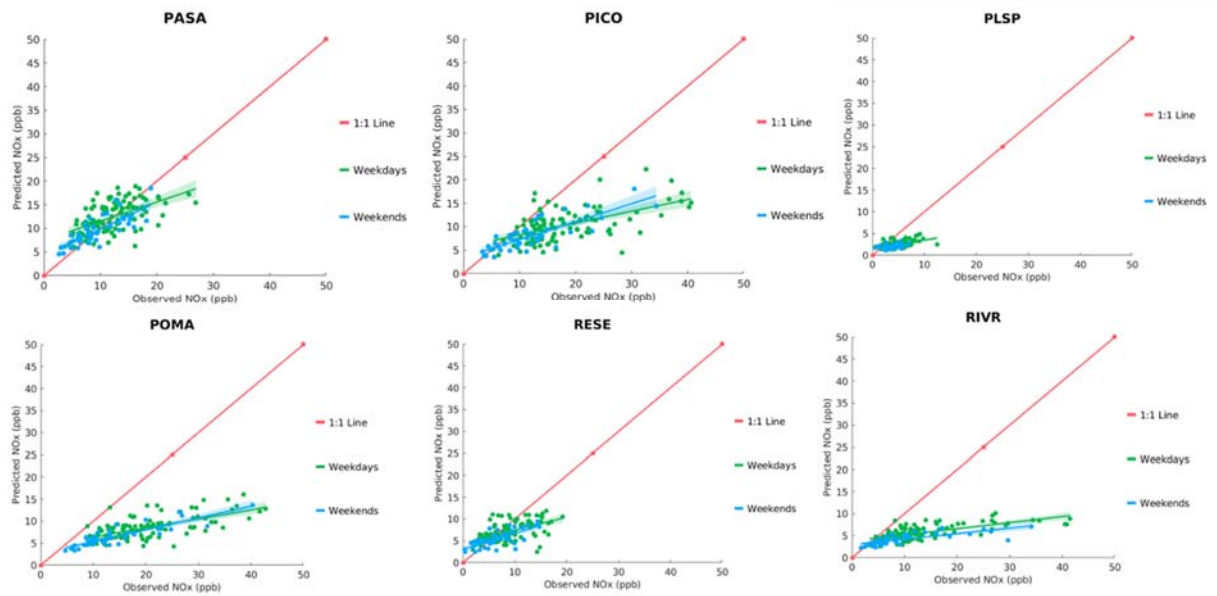
FIGURE N-3: SCATTER PLOT OF OBSERVED VS. PREDICTED DAILY AVERAGE NO x DURING MAY 1 ST TO SEPTEMBER 30 TH , 2018, AT PASADENA (PASA), PICO RIVERO (PICO), PALM SPRINGS (PLSP), POMONA (POMA), RESEDA (RESE), AND RIVERSIDE (RIVR). GREEN AND BLUE LINES INDICATE GENERAL LINEAR MODEL FIT WITH 95% CONFIDENCE INTERVAL (SHADED AREA). THE RED LINE INDICATES 1:1 LINE.
