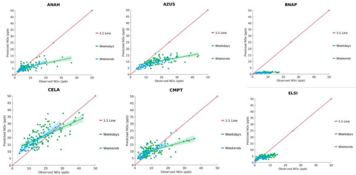
FIGURE N-1: SCATTER PLOT OF OBSERVED VS. PREDICTED DAILY AVERAGE NO x DURING MAY 1 ST TO SEPTEMBER 30 TH , 2018, AT ANEHIM (ANAH), AZUSA (AZUS), BANNING (BANP), COMPTON (CMPT), CENTRAL LOS ANGELES (CELA), AND LAKE ELSINORE (ELSI). GREEN AND BLUE LINES INDICATE GENERAL LINEAR MODEL FIT WITH 95% CONFIDENCE INTERVAL (SHADED AREA). THE RED LINE INDICATES 1:1 LINE.
