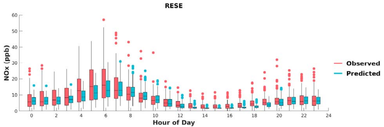
FIGURE I-17: BOX PLOTS OF OBSERVED VS. PREDICTED HOURLY NOX DURING MAY 1 ST TO SEPTEMBER 30 TH , 2018, AT RESEDA. HORIZONTAL LINES INDICATE 25 TH , 50 TH (MEDIAN), AND 75 TH PERCENTILES.
