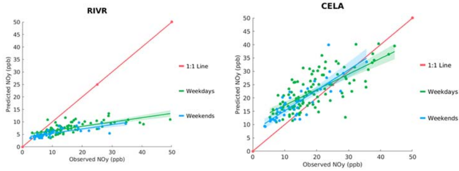
FIGURE O-1: SCATTER PLOT OF OBSERVED VS. PREDICTED DAILY AVERAGE NO y DURING MAY 1 ST TO SEPTEMBER 30 TH , 2018, AT RIVERSIDE (RIVR) AND CENTRAL LOS ANGELES (CELA). GREEN AND BLUE LINES INDICATE GENERAL LINEAR MODEL FIT WITH 95% CONFIDENCE INTERVAL (SHADED AREA). THE RED LINE INDICATES 1:1 LINE.
