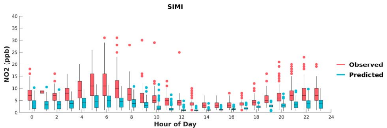
FIGURE H-20: BOX PLOTS OF OBSERVED VS. PREDICTED HOURLY NO2 DURING MAY 1 ST TO SEPTEMBER 30 TH , 2018, AT SIMI VALLEY. HORIZONTAL LINES INDICATE 25 TH , 50 TH (MEDIAN), AND 75 TH PERCENTILES.
