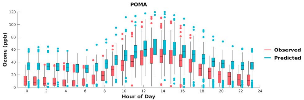
FIGURE F-21: BOX PLOTS OF OBSERVED VS. PREDICTED HOURLY OZONE DURING MAY 1 ST TO SEPTEMBER 30 TH , 2018, AT POMONA. HORIZONTAL LINES INDICATE 25 TH , 50 TH (MEDIAN), AND 75 TH PERCENTILES.
