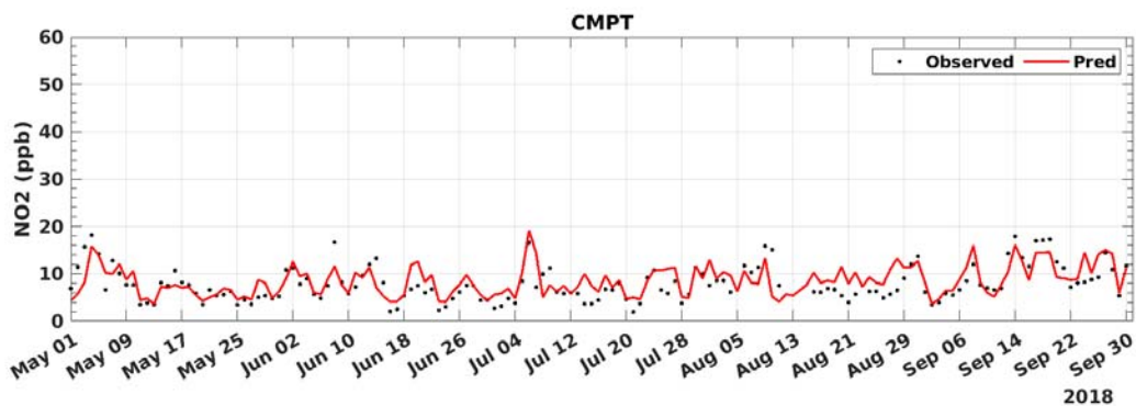
FIGURE C-5: 2018 DAILY AVERAGED NO2 MODEL PREDICTION AND MEASUREMENT COMPARISON AT COMPTON
