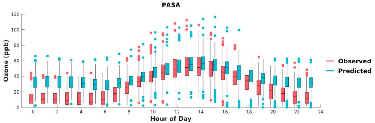
FIGURE F-17: BOX PLOTS OF OBSERVED VS. PREDICTED HOURLY OZONE DURING MAY 1 ST TO SEPTEMBER 30 TH , 2018, AT PASADENA. HORIZONTAL LINES INDICATE 25 TH , 50 TH (MEDIAN), AND 75 TH PERCENTILES.
