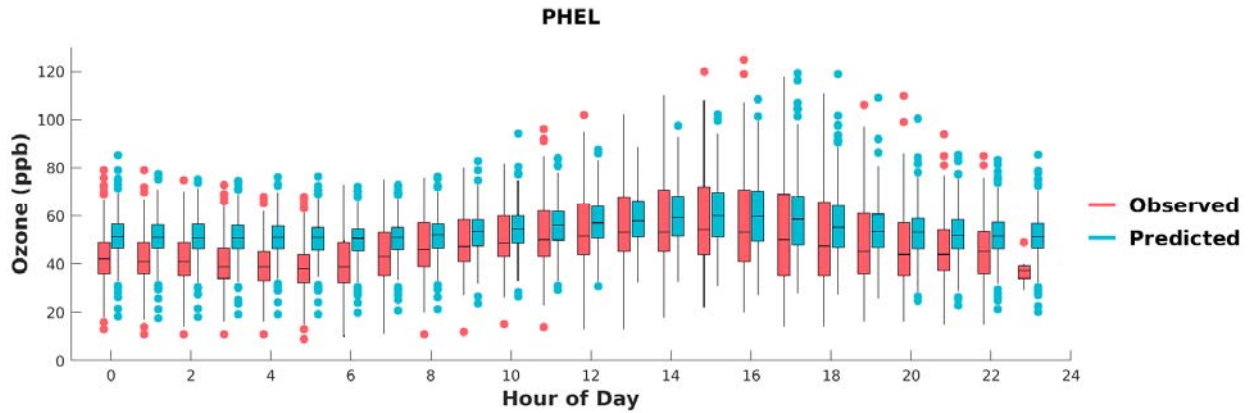
FIGURE F-19: BOX PLOTS OF OBSERVED VS. PREDICTED HOURLY OZONE DURING MAY 1 ST TO SEPTEMBER 30 TH , 2018, AT PHELAN. HORIZONTAL LINES INDICATE 25 TH , 50 TH (MEDIAN), AND 75 TH PERCENTILES.
