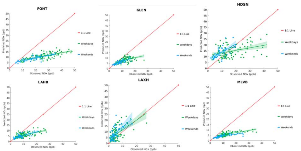
FIGURE N-2: SCATTER PLOT OF OBSERVED VS. PREDICTED DAILY AVERAGE NO x DURING MAY 1 ST TO SEPTEMBER 30 TH , 2018, AT FONTANA (FONT), GLENDORA (GLEN), HUDSON (HDSN), AND LA HABRA (LAHB), LAX (LAX), AND MIRA LOMA (MLVB). GREEN AND BLUE LINES INDICATE GENERAL LINEAR MODEL FIT WITH 95% CONFIDENCE INTERVAL (SHADED AREA). THE RED LINE INDICATES 1:1 LINE.
