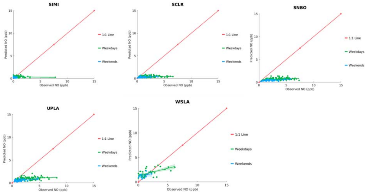
FIGURE L-4: SCATTER PLOT OF OBSERVED VS. PREDICTED DAILY AVERAGE NO DURING MAY 1 ST TO SEPTEMBER 30 TH , 2018, AT SIMI VALLEY (SIMI), SANTA CLARITA (SCLR), SAN BERNARDION (SNBO), UPLAND (UPLA), AND WEST LOS ANGELES (WSLA). GREEN AND BLUE LINES INDICATE GENERAL LINEAR MODEL FIT WITH 95% CONFIDENCE INTERVAL (SHADED AREA). THE RED LINE INDICATES 1:1 LINE.
