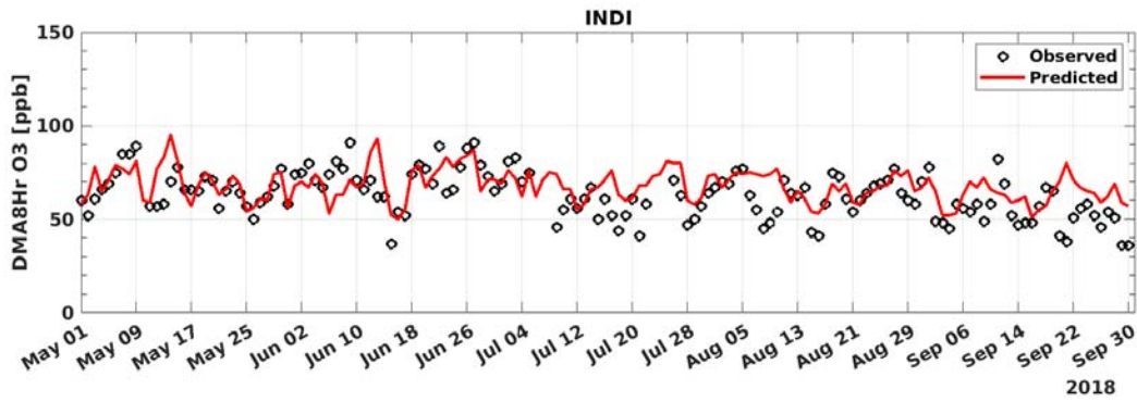
FIGURE A-10: 2018 MAXIMUM DAILY AVERAGE 8-HOUR (MDA8) OZONE MODEL PREDICTION AND MEASUREMENT COMPARISON AT INDIO
