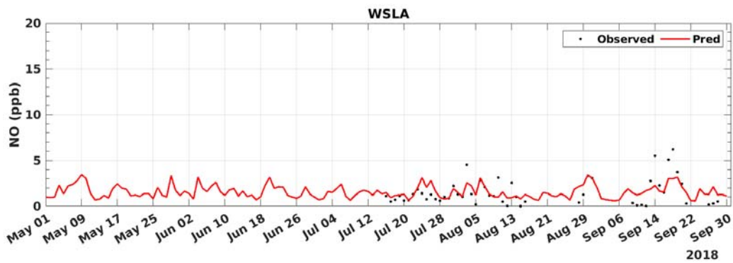
FIGURE B-27: 2018 DAILY AVERAGED NO MODEL PREDICTION AND MEASUREMENT COMPARISON AT WEST LOS ANGELES
