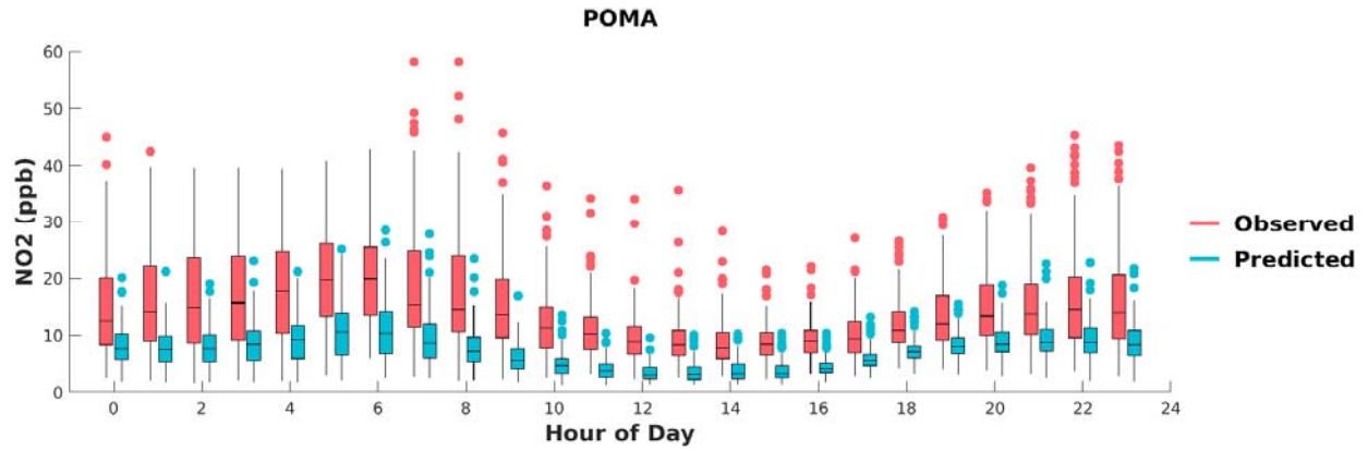
FIGURE H-15: BOX PLOTS OF OBSERVED VS. PREDICTED HOURLY NO 2 DURING MAY 1 ST TO SEPTEMBER 30 TH , 2018, AT POMONA. HORIZONTAL LINES INDICATE 25 TH , 50 TH (MEDIAN), AND 75 TH PERCENTILES.
