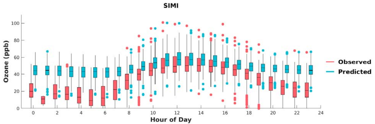
FIGURE F-27: BOX PLOTS OF OBSERVED VS. PREDICTED HOURLY OZONE DURING MAY 1 ST TO SEPTEMBER 30 TH , 2018, AT SIMI VALLEY. HORIZONTAL LINES INDICATE 25 TH , 50 TH (MEDIAN), AND 75 TH PERCENTILES.
