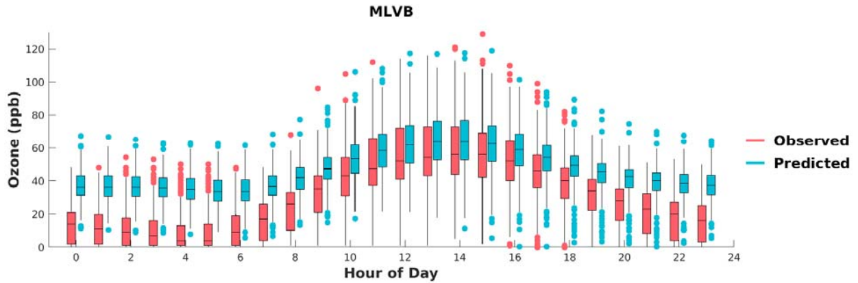
FIGURE F-15: BOX PLOTS OF OBSERVED VS. PREDICTED HOURLY OZONE DURING MAY 1 ST TO SEPTEMBER 30 TH , 2018, AT MIRA LOMA VAN BUREN. HORIZONTAL LINES INDICATE 25 TH , 50 TH (MEDIAN), AND 75 TH PERCENTILES.
