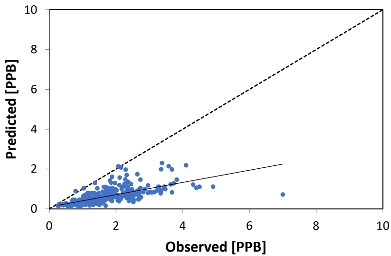
Figure 7. Scatter Plot of Predicted vs. Observed Concentrations Acetaldehyde
