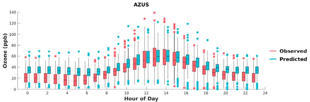
FIGURE F-2: BOX PLOTS OF OBSERVED VS. PREDICTED HOURLY OZONE DURING MAY 1 ST TO SEPTEMBER 30 TH , 2018, AT AZUSA. HORIZONTAL LINES INDICATE 25 TH , 50 TH (MEDIAN), AND 75 TH PERCENTILES.
